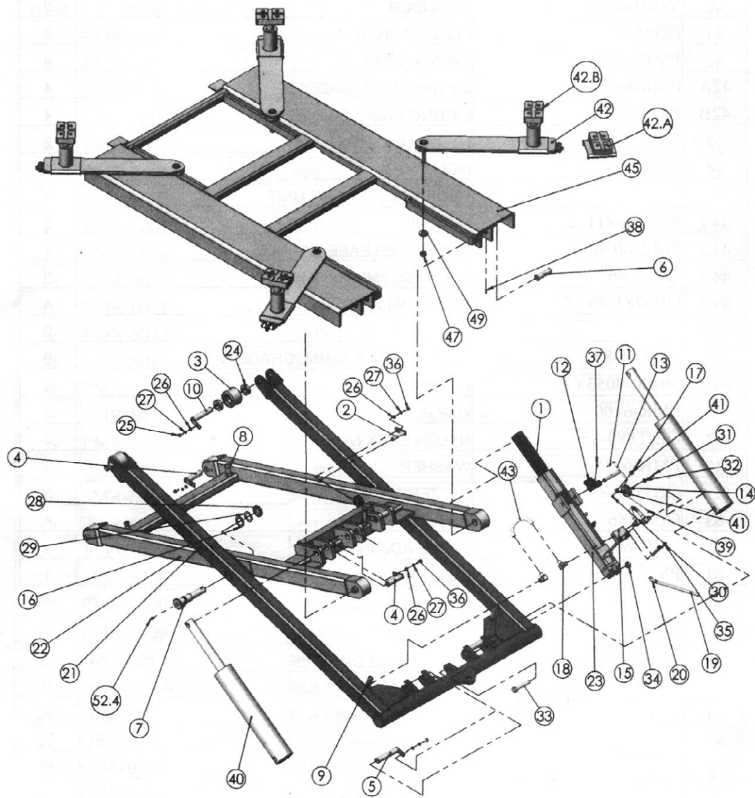
Figure 5-1. Illustrated Parts Breakdown – Sheet 1 of 3
